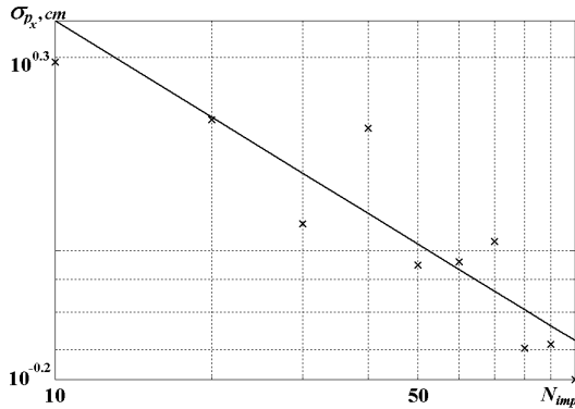
Fig. 6. Mean-square error of distance estimation along axis x (straight line is theoretical estimation, (x) is experimental results) depending on a number of pulses in the pack. The duration of radio pulse is 10 ns.
