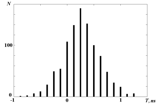
Fig. 3. Distribution of central point of interval between t_1 and t_2 relative to exact arrival time of chaotic radio pulse
