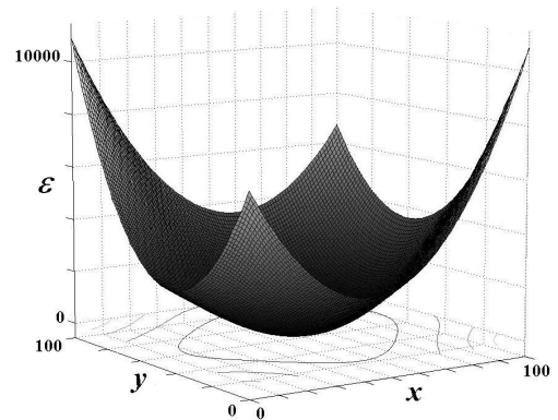
Fig. 5. Functional \varepsilon as a function of coordinates x and y . The minimum correspond to the coordinates of the transmitter
