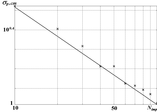
Fig. 4. Mean-square error of distance estimation (straight line is theoretical estimation, (x) is experimental results) as a function of the number of pulses in pack. The duration of radio pulse is 10 ns.
