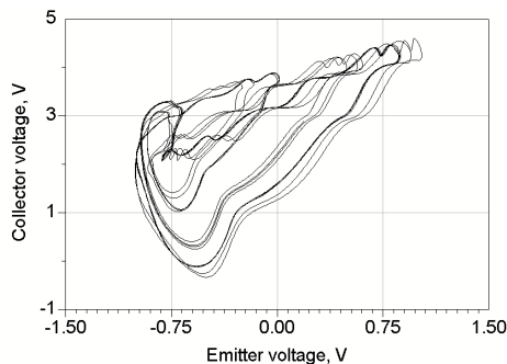
Fig. 10. Fragment of phase portrait of three-point scheme with BFP620 transistor.
