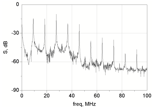
Fig. 7 (c). Frequency range – megahertz. \gamma = 2000 .
