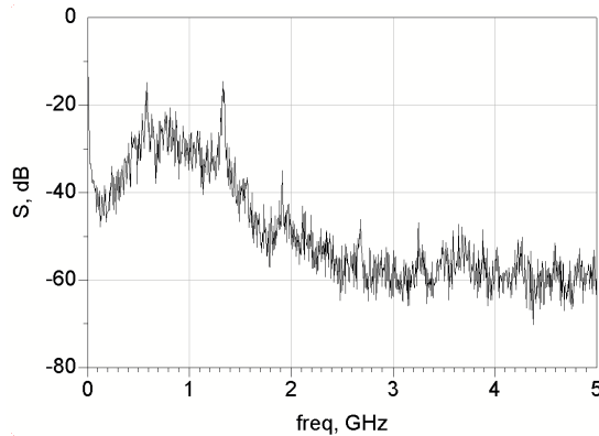
Fig. 9. Power spectrum in three-point circuit with BFP620 transistor.
