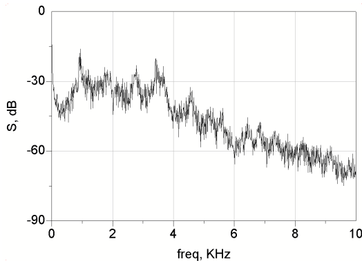
Fig. 7 (a). Power spectrum in three-point circuit with Gummel-Poon model of BFP620 transistor. Frequency range – kilohertz. \gamma = 2 .
