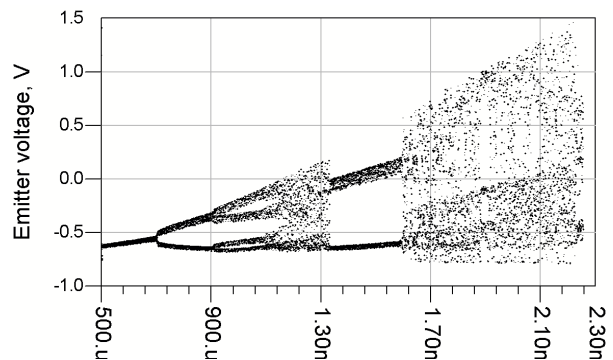
Fig. 8. Bifurcation diagram for three-point scheme with Gummel-Poon model of BFP620 transistor. Frequency range – megahertz.
