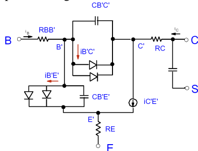
Fig. 3. Equivalent circuit for Gummel-Poon model.
