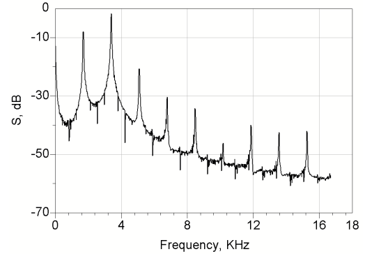
Fig. 4. Power spectrum in three-point circuit with SPICE model of 2N2222 transistor. Frequency range – kilohertz.
