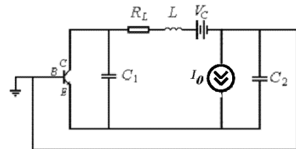
Fig. 1. Three-point scheme of generator with current source in emitter circuit.
