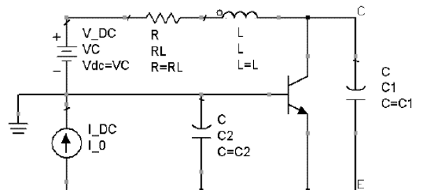
Fig. 2. Three-point scheme of generator. Representation in ADS.
