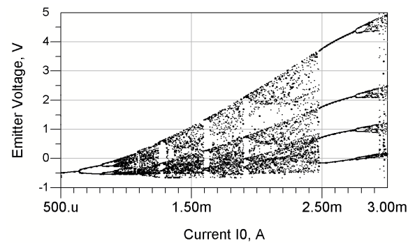
Fig. 5. Bifurcation diagram for three-point scheme with the model with exponential characteristics for 2N2222 transistor. Frequency range – kilohertz.
