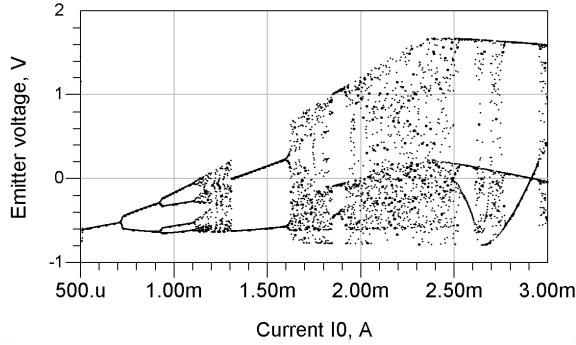
Fig. 6. Bifurcation diagram for three-point scheme with Gummel-Poon model of BFP620 transistor. Frequency range – kilohertz.
