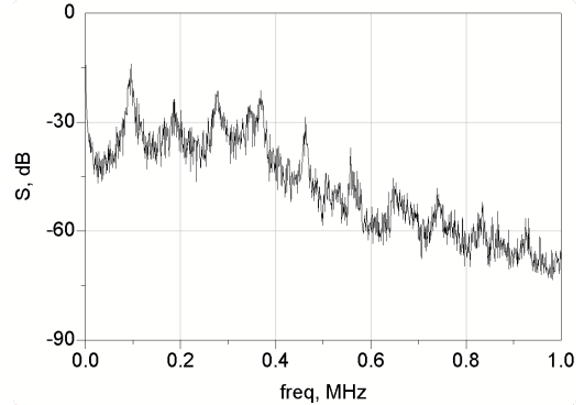
Fig. 7 (b). Frequency range – hundreds of kilohertz. \gamma = 200 .
