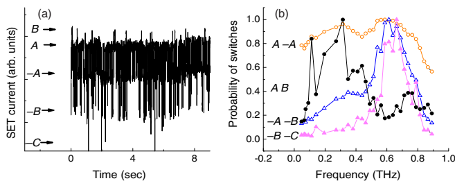
FIG. 5. (a) Time traces of SET current at 0.8 THz. There are few levels corresponding to different QD states: ground A and -A , excited B and -B , double excited -C . (b) Switches between different states normalized to maximum counts: AB switches have a maximum at 0.3 THz, -A -B and -B -C have a maximum at 0.7 THz, and A - A has both resonances.
