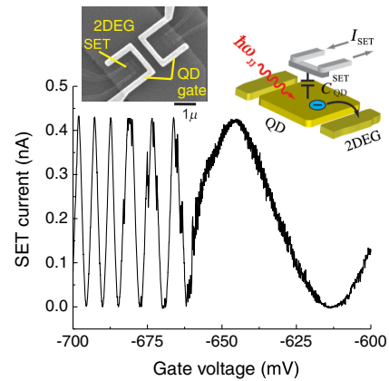
FIG. 2. CBO of the aluminum SET as a function of voltage on the QD gate. The CBO period changes at V_G \sim -0.654 \text{ V} when the QD is formed in the 2DEG. Inset: A SEM picture and operation scheme of the detector. The QD is formed in the 2DEG by the negatively biased QD gate and the edge of the mesa strip. The QD is capacitively coupled to the aluminum SET fabricated on top of the mesa strip. The SET current is sensitive to the excitation of electrons out of the QD upon absorption of terahertz photons.
