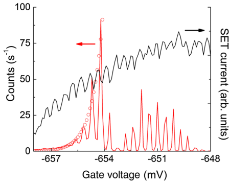
FIG. 3. Count rate of charge excitation of the QD due to thermal photons at T = 0.02 K. Oscillations of the count rate are correlated with the CBO of the QD seen in the SET current. Counts are suppressed below V_G \sim -0.657 V when the QD is completely decoupled from the surrounding 2DEG. Open circles are the exponential fit of the suppression
