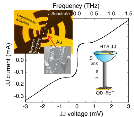
FIG. 1. I - V curve of a HTS JJ taken at 0.02 K. Top axis is the Josephson frequency corresponding to the voltage across the JJ. Insets: Optical image of a 2- \mu\text{m} -wide HTS JJ defined at the bicrystal boundary and the optical scheme of the experiment.
