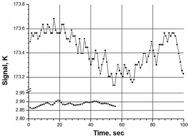
Fig. 6.7 Time dependence of the lock-in output for different levels of the receiver input signal for receiver T4m-093#6m. The input signal is the difference between the temperatures of the chopper blades and the load. In the case of a large difference ( top line ) NETD = 143 ± 14 mK, and for a small difference ( bottom line ) NETD = 10 ± 1 mK. In both cases the integration time of the lock-in amplifier was 1 s
