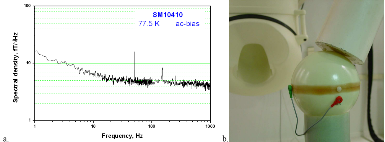
Fig. 1. (a) Noise spectral density of the 16-mm high- T_c magnetometer; (b) photograph taken during the test measurement with head phantom by the high- T_c system.
