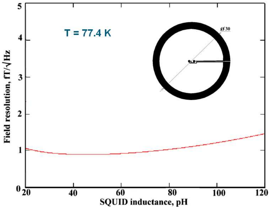
Fig. 4. Expected magnetic field resolution B_N(L_S) of high- T_c DC SQUID magnetometer consisted of a dual-SQUID inductively coupled to 30-mm superconducting flux transformer (see insert) having two multiturn input coils.
