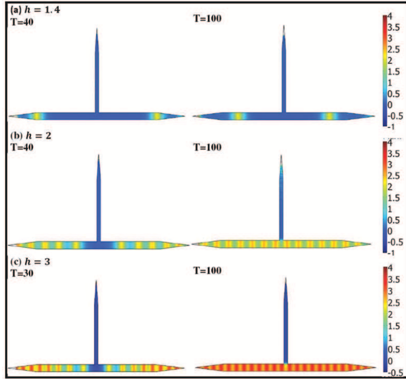
Fig. 3 Numerical simulations for the penetration of magnetic flux into junction without applied bias current. (a) At h = 1.4 , only one vortex can enter from each boundaries A and G. They penetrate a small distance into the junction and then are pinned. (b) At h = 2 , many vortices can pass through the junction. At T-junctions, these vortices are bonded and are not cloned. (c) At h = 3 , the penetrated vortices are moved fast. The concentration of fluxons in the junction also increases. Vortex fission does still not occur. The colour scale represents the distribution of the magnetic field from -0.5 to 4.
