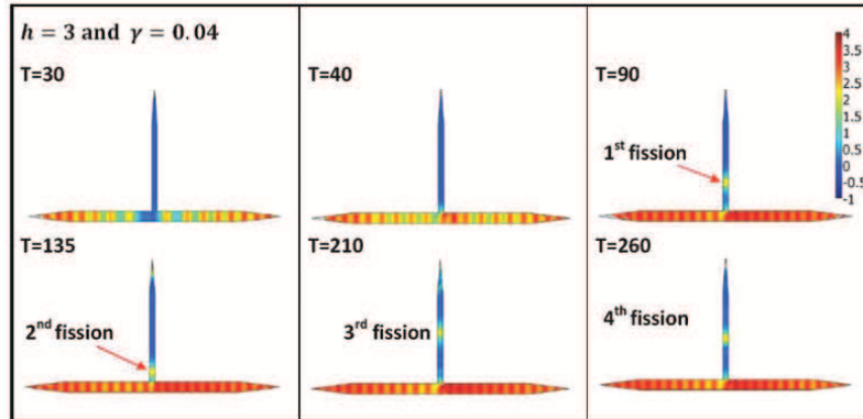
Fig. 5 Numerical simulations of magnetic flux penetration into the junction when h=3 and \gamma=0.04 . In main FFO, fast vortices enter from each boundaries A and G and move toward T-junction. Vortices on the left side are continued to move toward T-junction without stopping (no pinning is observed). Because of speedy vortices originated from the right side, they pass through T-junction and continue moving to the left with pushing vortices on left side and moving to left direction. Succession divisions are a bit faster than in the case h=2 in Fig. 4 (a). The colour scale represents the distribution of the magnetic field.
