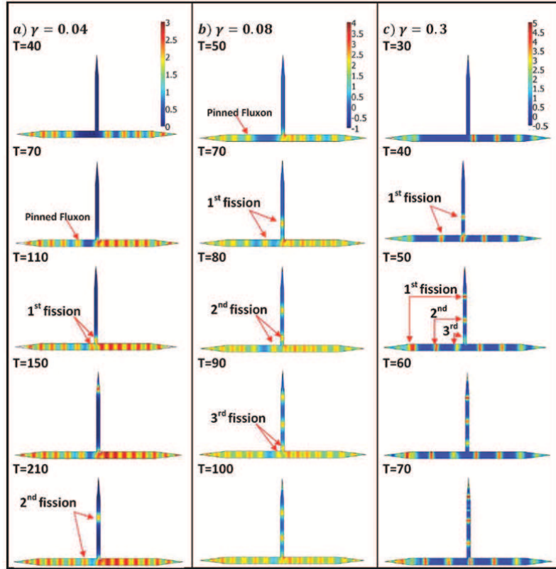
Fig. 4 Numerical simulations for penetration of magnetic flux into junction when variable bias current at h = 2 . (a) At \gamma = 0.04 , the most vortices are entering from the right side of the main FFO. On left side of the main FFO, they struggle to approach the T-junction. Then, they are pushed to right by cloned vortices, which enter from T-junction. Vortex fission occurs slowly. (b) At \gamma = 0.08 , the acceleration of vortices from the right side increases while the vortices from the left side slowdowns. The flowing of vortices and thier fission take less time. (c) At \gamma = 0.3 , vortices in main FFO flow from the right to the left. There are flontly in vortex fission. The colour scale represents the distribution of the magnetic field.
