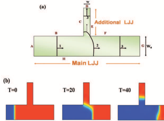
Fig. 1 (a) A schematic picture of the vortex positions in the T-shape Josephson junction (presented in the bold lines) during the vortex nucleation process. The thin arrows indicate the direction of the vortex motion. The vortex state before nucleation is denoted by 1; the moment of nucleation is denoted by 2; the vortex state after the nucleation is denoted by 3. Widths of main and additional branches of the T-junction are W_0 and W , respectively (b) Division of the vortex moving with velocity higher than the critical. Widths of the main and additional branches of the T-junction are W_0 = 10 and W = 5 \lambda_J respectively, where \lambda_J is a Josephson length. The blue and red colours are two equivalent states of a superconductor without vortices.
