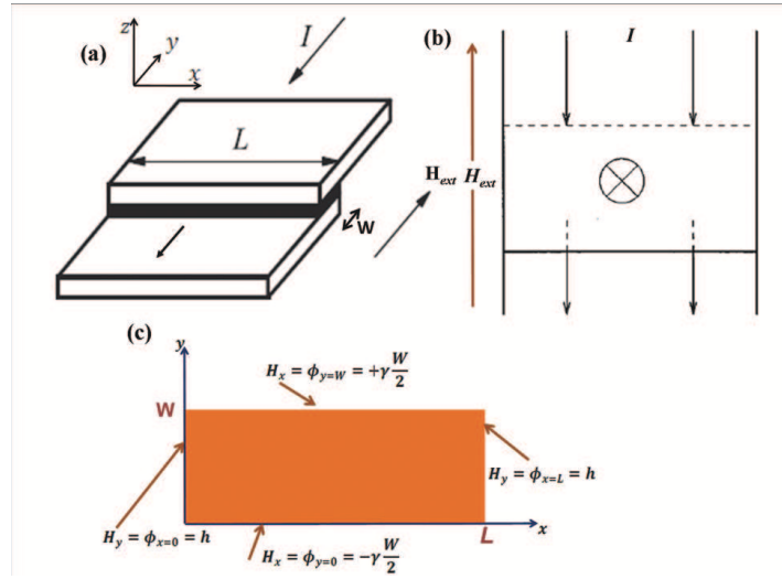
Fig. 2 (a) Josephson tunnel junction of overlap type. (b) Schematic diagram top of the overlap LJJ. The current from the upper electrode goes through the junction and comes in the lower electrode. (c) Overlap boundary conditions for the 2D sine-Gordon equation. The magnetic field, bias current and all lengths are dimensionless.
