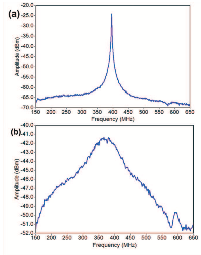
Fig. 7 FFO spectra associated with radiation emitted by additional LJJ. (a) frequency - 216 GHz, linewidth - 1.4 MHz. (b) FFO frequency - 716 GHz, linewidth - 130 MHz.
