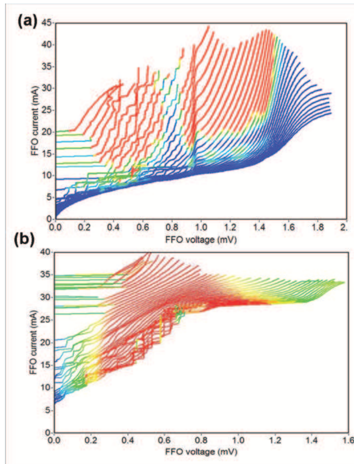
Fig. 6 (a) Experimental measured IVCs for conventional FFO at different magnetic fields created by current applied to integrated control line. (b) IVCs of the FFO with flux cloning circuits at different magnetic fields created by current applied.
