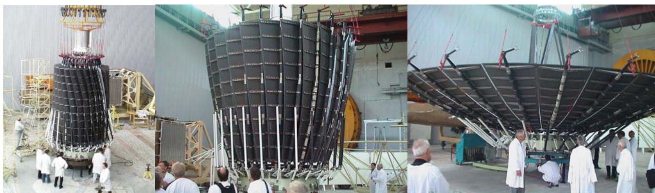
Fig. 2 Different stages of the "RadioAstron" 10m antenna deployment at Lavochkin Association (Moscow, Russia).
