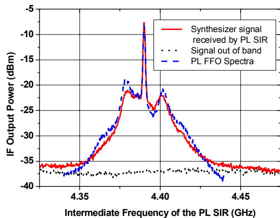
Fig. 14. Signal of multiplier driven by synthesizer ( 17.967 \text{ GHz} \times 37 = 664.8 \text{ GHz} ), measured by TELIS SIR with FFO phase-locked at 660.4 \text{ GHz} – solid line. For the trace shown by dotted line the signal of the synthesizer is shifted by 5 \text{ MHz} to be out of IF band. Dashed line – spectrum of the PL FFO, measured at HM IF output and frequency translated.
