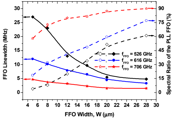
Fig. 8. Linewidth of free-running FFOs (left axis) and corresponding Spectral Ratio for the phase-locked FFO (right axis) measured at different FFO
