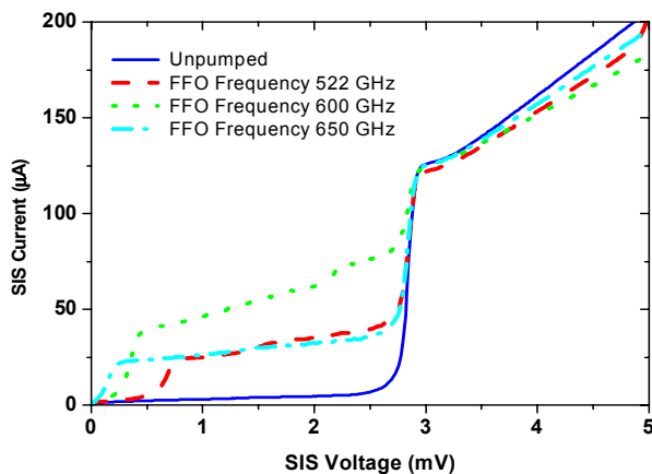
Fig. 5. IV-curves of the SIS-mixer: solid line - unpumped, dashed, dotted and dash-dotted - pumped by FFO at frequencies 522, 600 and 650 GHz correspondingly.
