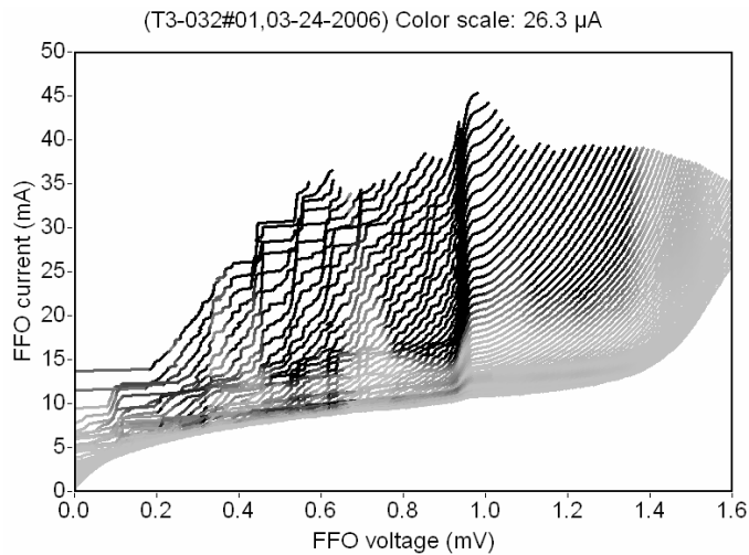
Fig. 4. IV-curves of the FFO (length = 400 \mu\text{m} , width = 16 \mu\text{m} ) measured at different FFO CL currents; the pumping of the SIS-mixer is shown by gray scale (black color corresponds to pumping level > 25% of SIS I_g ), see Fig. 5.
