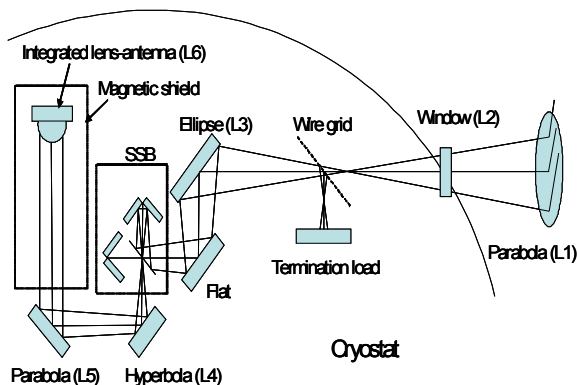
Fig. 1. Layout of the cold channel optics. Lines show the optical beam trajectories.
