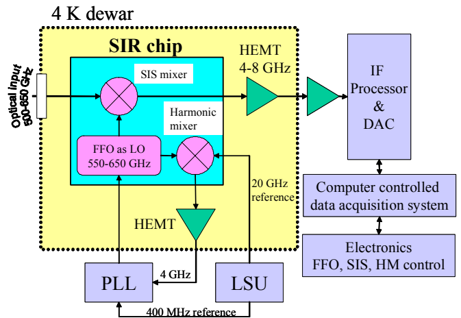
Fig. 2. Schematics of the SIR with phase-locked LO. FFO frequency is mixed in HM with the 19-21\ \text{GHz} reference. The mixing product is amplified, down converted and compared with the 400\ \text{MHz} reference in the PLL. The phase difference signal generated by PLL is used to feedback the FFO control line.
