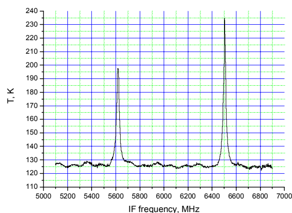
Fig. 15. Deconvolved spectrum of the OCS emission lines measured at different sidebands of the receiver at a gas pressure 1.2 \text{ mBar} . LO frequency 625.24 \text{ GHz} . Lines are saturated, the difference in line strength reflects the sideband ratio of the receiver.
