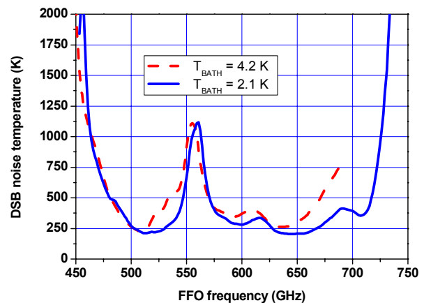
Fig. 10. Uncorrected DSB noise temperature of the SIR as a function of FFO frequency measured at different FFO bias currents to optimize the SIS pumping level: T_{\text{BATH}} = 2.1 \text{ K} (solid line), 4.2 \text{ K} (dashed line), V_{\text{SIS}} = 2.2 \text{ mV} , \text{IF} = 4.3 \text{ GHz} .
