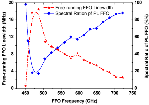
Fig. 7. Free-running linewidth and SR of PL FFO as a function of FFO frequency (FFO width = 28 \mu\text{m} ; R_n S = 30 \text{ Ohm} \cdot \mu\text{m}^2 ).
