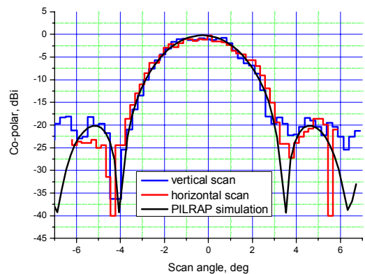
Fig. 11. Vertical (blue curve) and horizontal (red curve) far-field scans. The fit (black curve) is diffraction pattern calculated by PILRAP [11].
